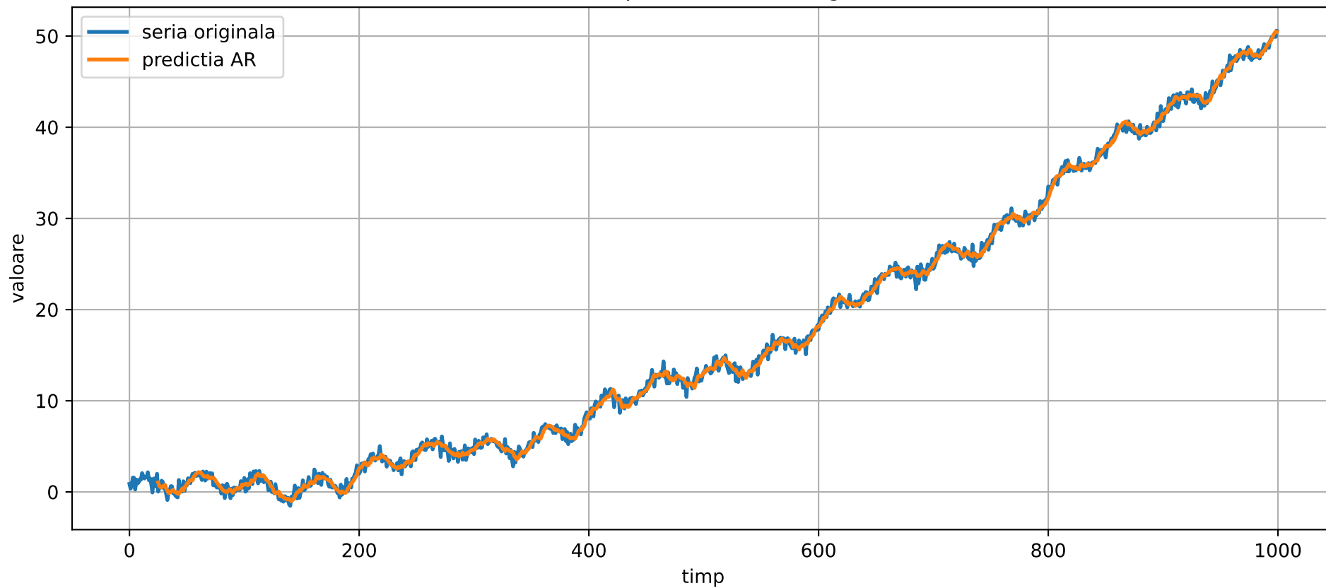
Model AR(p=25) vs seria originala
